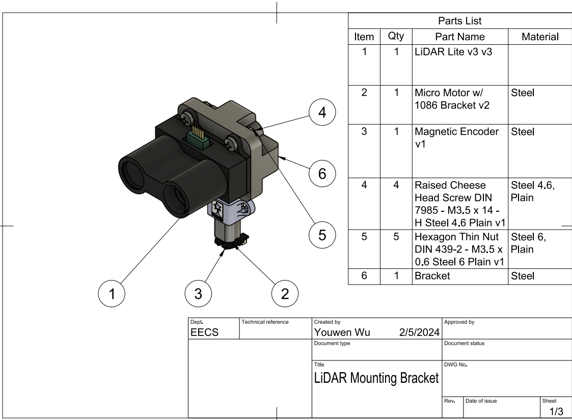
Figure 3: Parts Diagram
