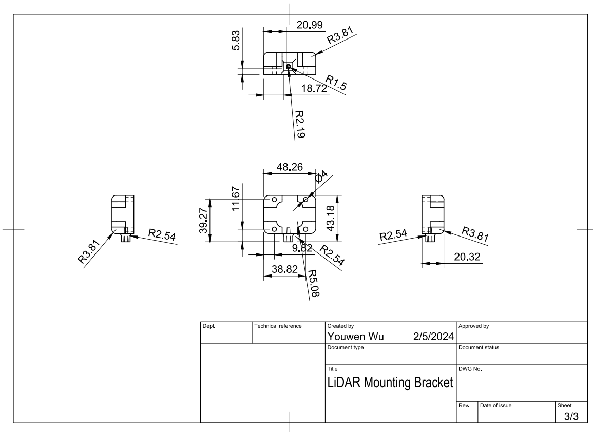
Figure 4: Engineering Drawings
